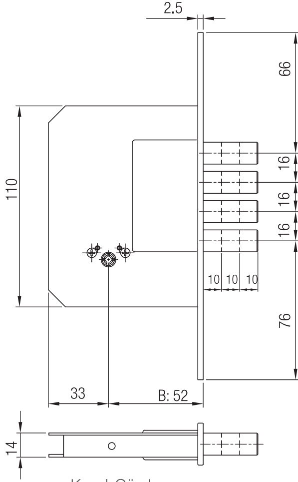
Kapalı Gövde Closed case
