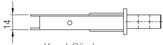
Kapalı Gövde Closed case
